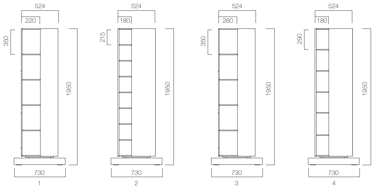
Atlas Single H:195 cm
