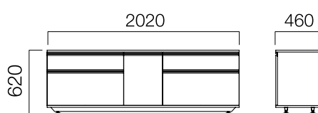
Cabinet 4 Drawers 1 Lid
