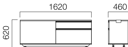
Double Sided Commode 4 Drawers
