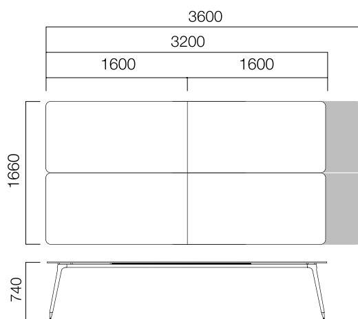
W:166 cm 4-Set Meeting Table
