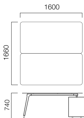
W:166 cm 2-Set Double-Leg Meeting
