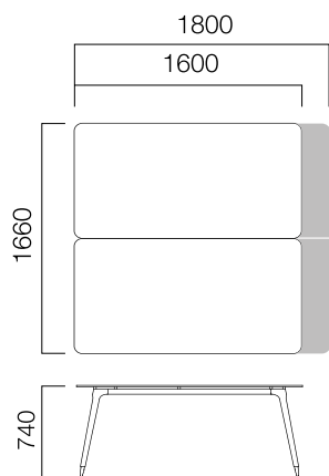
W:166 cm 2 Set Meeting Table
