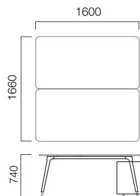
W:166 cm 2-Set Triple-Leg Meeting Table
