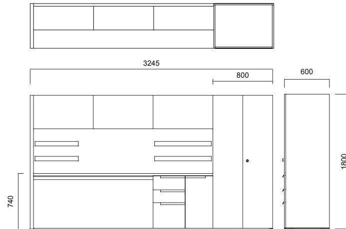
Private Office Cabinet 2
