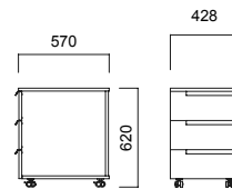
Private Office Mobile Pedestal
