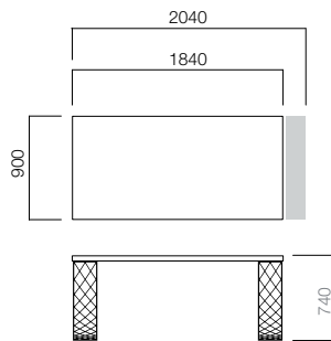
Desk w/ 2 Legs
