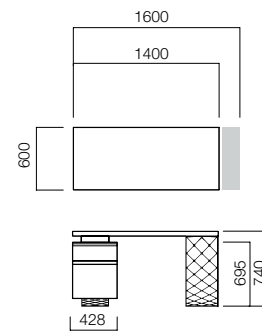
Side Desk w/ Pedestal
