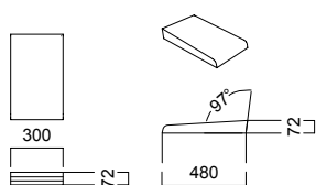
To Cushion
